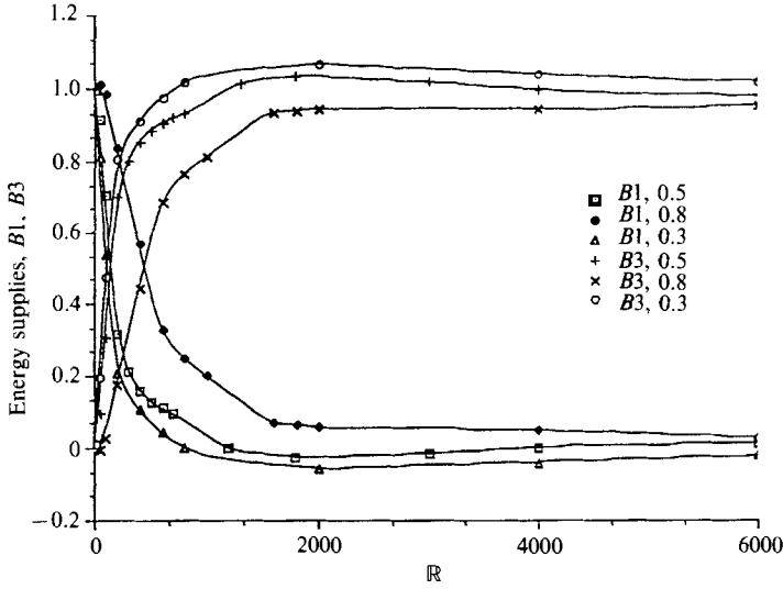
FIGURE 13. Energy supply B1, B3 for a = 1.1, m = 1, F = 0, J^* = 2000 and \zeta_2 = 0.8, 0.5, 0.3 . At large Reynolds numbers, interfacial gravity B3 is the main source of instability.
