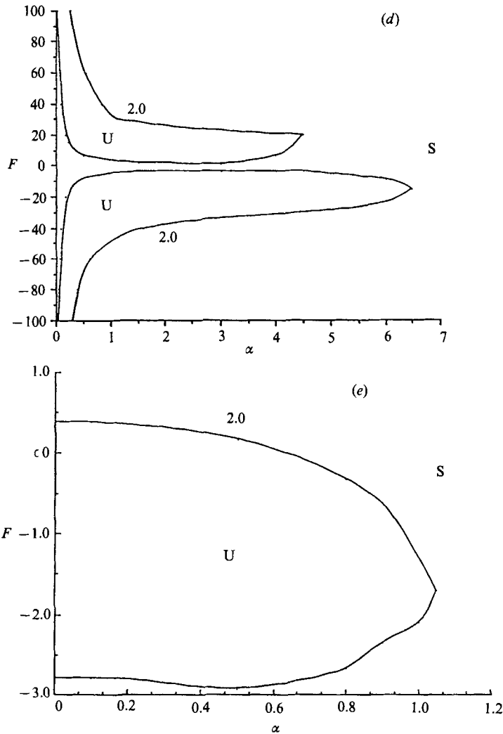
FIGURE 24. Neutral curves for a = 1.4 , m = 0.5 , J^* = 2000 , Re = 10 and various \zeta_2 . (a) Left branch for \zeta_2 = 0.5 . (b) Right branch for \zeta_2 = 0.5 . CAF is always unstable. (c) \zeta_2 = 1 . CAF is always unstable. (d) Positive and negative upper branches for \zeta_2 = 2 . There is a narrow band of stability. (e) Region of capillary instability for \zeta_2 = 2 .
