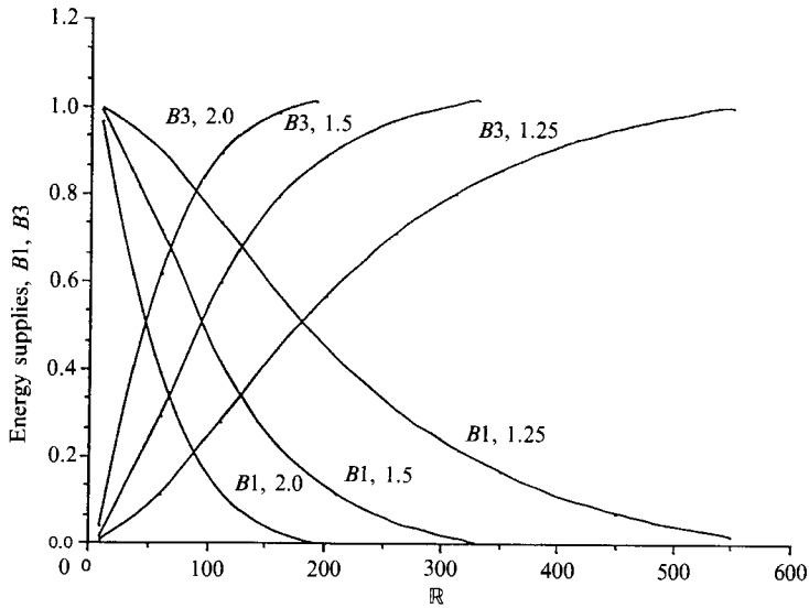
FIGURE 10. Energy supply B1, B3 for a = 1.1 , m = 1 , F = 0 , J^* = 2000 , \zeta_2 = 2.0, 1.5, 1.25 . Interfacial gravity B3 is always positive, destabilizing the flow.
