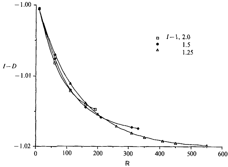
FIGURE 11. I-D for a = 1.1 , m = 1 , F = 0 , J^* = 2000 , \zeta_2 = 2.0, 1.5, 1.25 .
