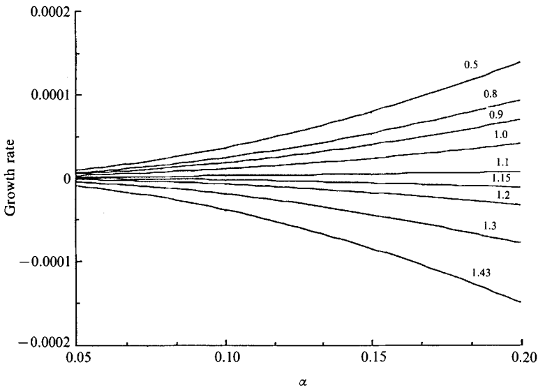
FIGURE 8. Growth rates for a = 1.86 , m = 0.5 , J^* = F = 0 , \mathbb{R} = 1 , and various values of \zeta_2 indicated above each curve. The JRR long-wave instability ( \zeta_2 = 1 ) is reinforced when \zeta_2 < 1 , suppressed when \zeta_2 > 1 and stabilized when \zeta_2 \geq 1.15 .
