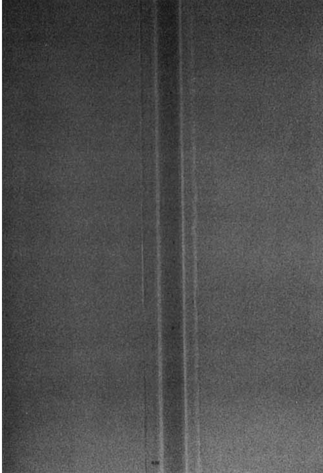
FIGURE 3. Stable perfect core-annular flow of SAE 30 oil and glycerine/water mixture. a = 1.86 , m = 0.33 , \zeta_2 = 1.4 , J^* = 2.26 , F = 0 , \mathbb{R}_y = 1.82 .
