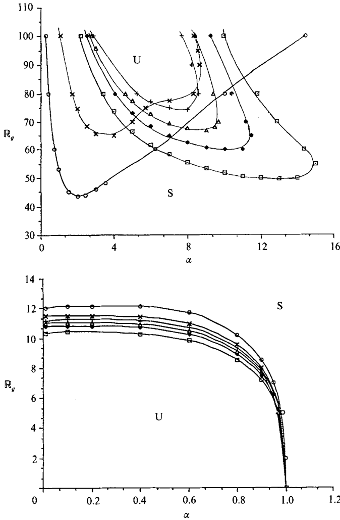
FIGURE 16. Lower and upper branches of the neutral curves for a = 1.1 , m = 0.5 , F = 0 , J^* = 2000 , \zeta_2 = 2.0, 1.6, 1.4, 1.2, 1.0, 0.5 . Stable and unstable regions are marked by S and U respectively. The plotting symbols for \zeta_2 are: \square , 2.0; \blacklozenge , 1.6; \triangle , 1.4; + , 1.2; \times , 1.0; \circ , 0.5.
