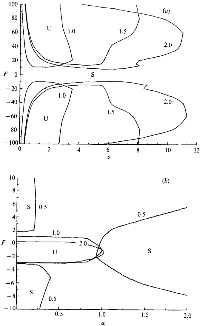
FIGURE 22. Neutral curves for a = 1.2 , m = 0.5 , J^* = 2000 , R_p = 10 , and different values of \zeta_2 . (a) Positive and negative F upper branches. The stability regions are largest when the density ratio \zeta_2 is close to 1.5. (b) Detailed view near the capillary instability region. The neutral curves for \zeta_2 = 0.5 are also shown here. CAF is always unstable for \zeta_2 = 0.5 .
