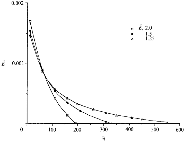
FIGURE 9. The rate of change of disturbance energy \dot{E} vs. Reynolds number R for a = 1.1 , m = 1 , F = 0 , J^* = 2000 , \zeta_2 = 2.0, 1.5, 1.25 . The flow is stable when R > R_c(\zeta_2) : R_c(2.0) = 190 , R_c(1.5) = 330 , R_c(1.25) = 550 .
