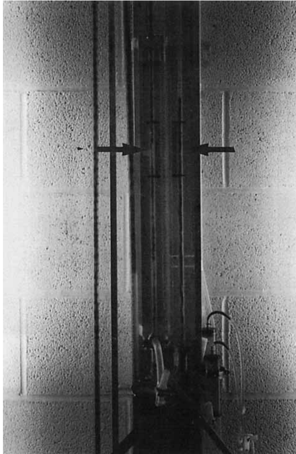
FIGURE 5. Forced-flow apparatus. The sections indicated by arrows are test sections and they are surrounded by boxes filled with glycerine to eliminate visual distortion. The left test section is for up-flow and the right is for down-flow. The two extra sections on the far left are only used for demonstration purpose. The inner radius of the pipe is 0.48 cm.
